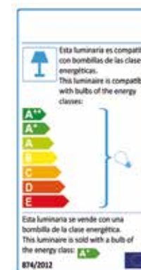
△ 662514 7449 Puntos/points 990 ↔ 43 ↑ 172 ↘ 43 cm 1 E27 LED 10W 900 lumen / 3.000 K Peso/weight 8,6 Kg
