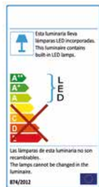
△ 825306 △ Puntos/points 450 ↔ 75 ↑ 155 ↘ 27 cm 20W LED 1.400 lumen / 4.000 K Peso/weight 2,55 Kg
