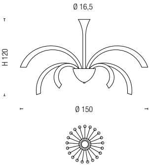
2031/21 CE 21 x max 25W G9
