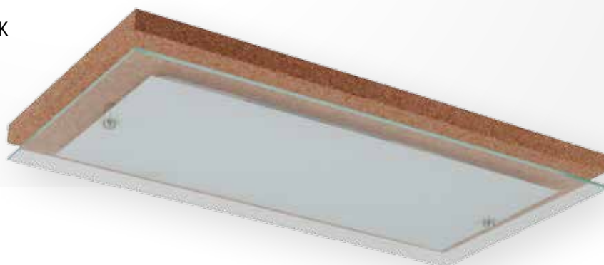
Item no. 4032974 ↔ 570 ↗ 290 ↓ 65 mm incl. 1xLED 24W, 2100lm, 2700K
